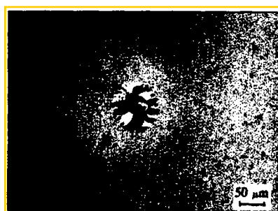
Fig. 10. Nomarski interference contrast in optical micrograph of a typical pit on implanted steel surface.
