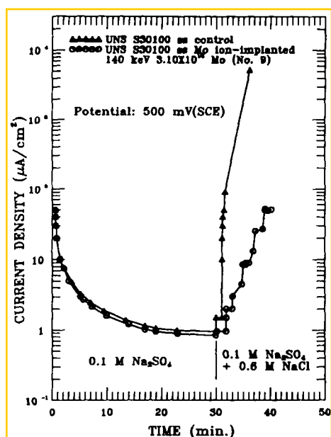
Fig. 4. Current density as a function of time, before and after the addition of chloride ions, for a control sample and implanted alloy sample #9 (Table 2).
