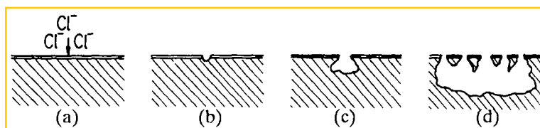
Fig. 11. Schematic development of "lacy" pits by undercutting mechanism.
